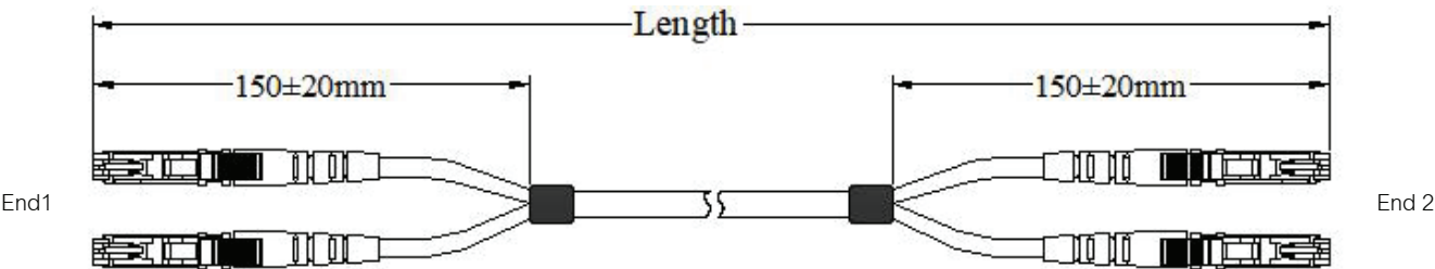
E2000 2.0mm&3.0mm duplex patchcord
